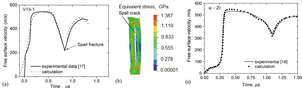
Fig.4. (a) Shock wave profiles in Ti-5Al-2.5Sn; solid curve is the experimental data [17], dashed curve is calculated data; (b) the distribution of the equivalent stress near spall crack at it's formation of in the Ti-5Al-2.5Sn; (c) shock wave profiles in Zr (b); solid curve is the experimental data [18], the calculated data is shown by dashed curve.
