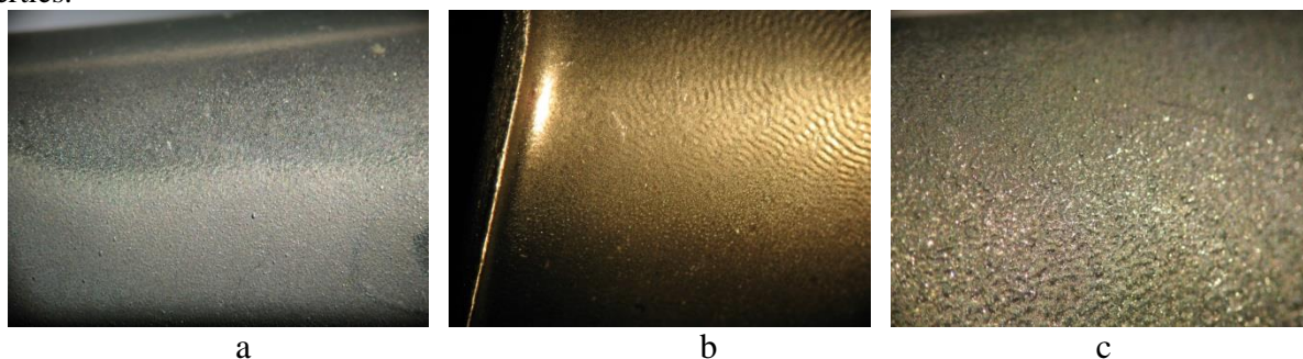
Fig.1 Topography of the turbine blade pen after various irradiation modes: a) 28,4 J/cm 2 , n=5; b) 34,6 J/cm 2 , n=5; c) 44,4 J/cm 2 , n=5.
